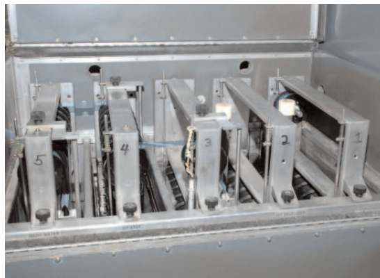
Developing Tank
